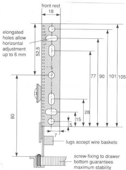
Position of mounting holes
